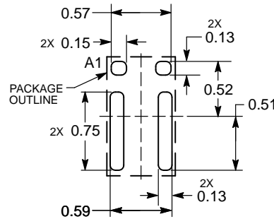
DIMENSIONS: MILLIMETERS
